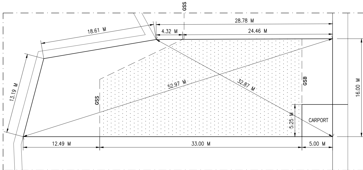
DENAH KAVLING JL.MAYANGPADMI KULON NO.47 SKALA 1 : 300
